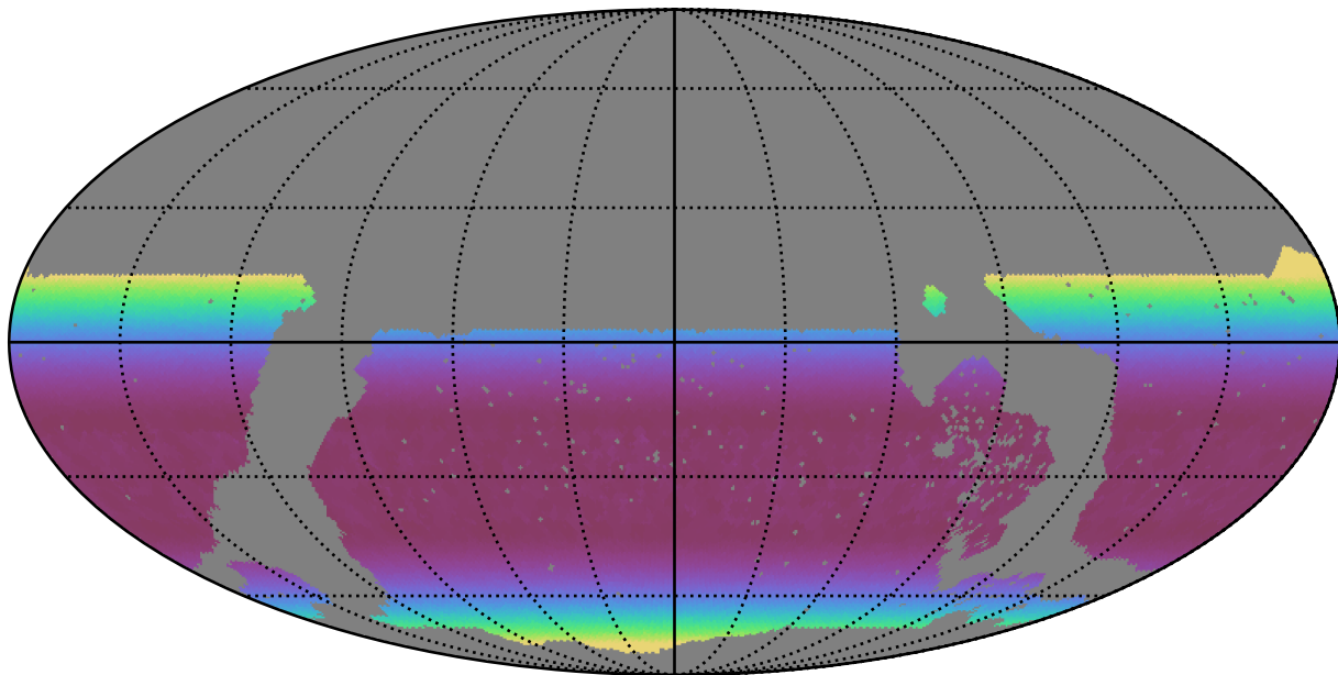
noroll_mjdp120_v3.4_10yrs WFD y band: Min airmass
