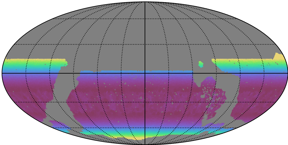
noroll_mjdp120_v3.4_10yrs WFD u band: Min airmass
