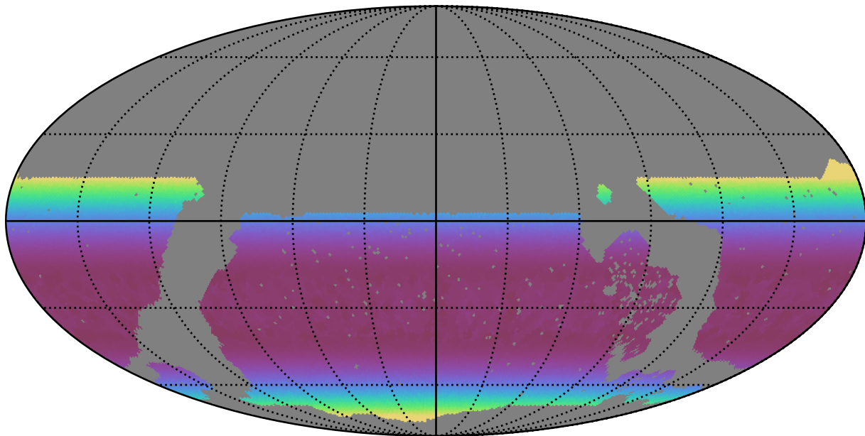
noroll_mjdp120_v3.4_10yrs WFD r band: Min airmass
