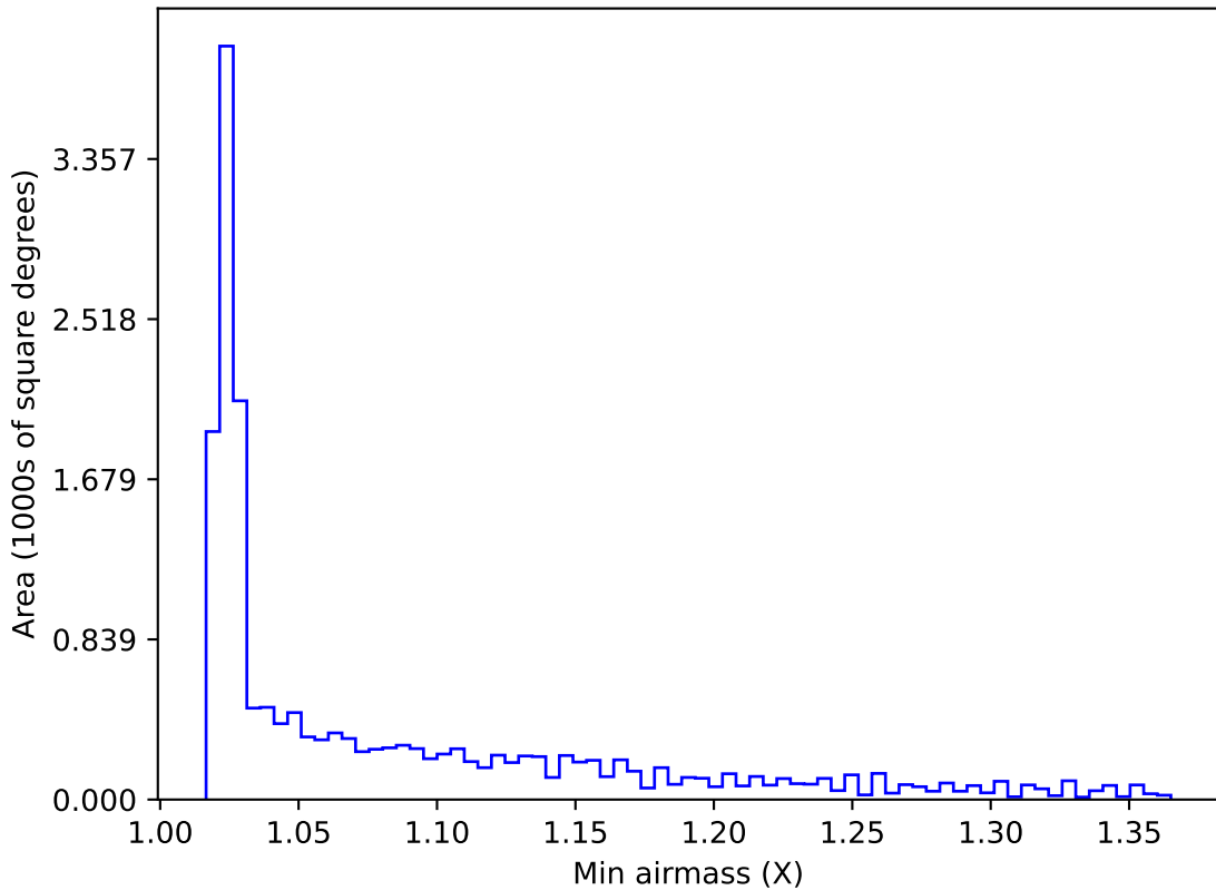
noroll_mjdp120_v3.4_10yrs WFD all bands: Min airmass
