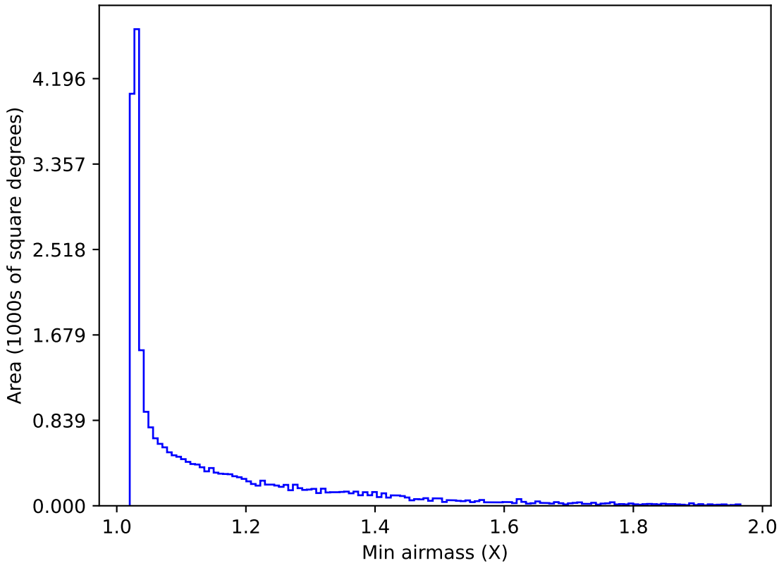
noroll_mjdp120_v3.4_10yrs All sky z band: Min airmass
