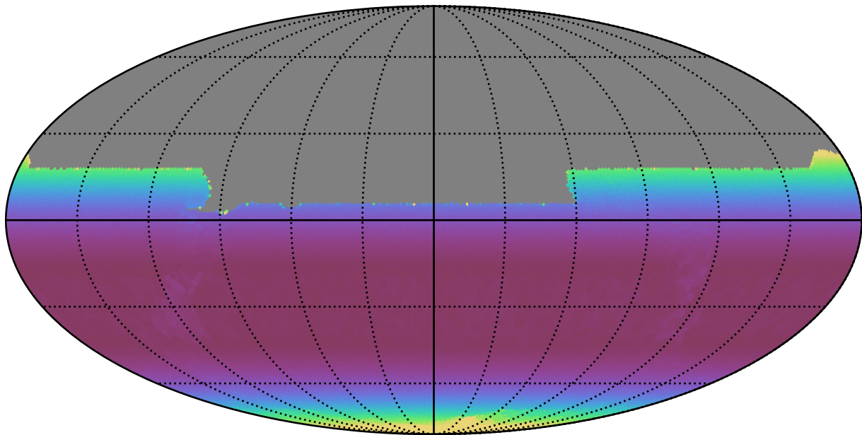
noroll_mjdp120_v3.4_10yrs All sky y band: Min airmass
