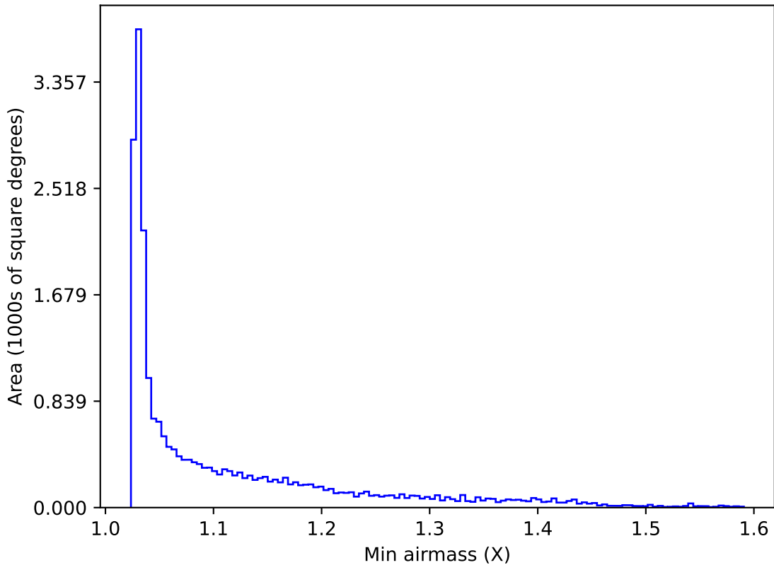
noroll_mjdp120_v3.4_10yrs All sky y band: Min airmass
