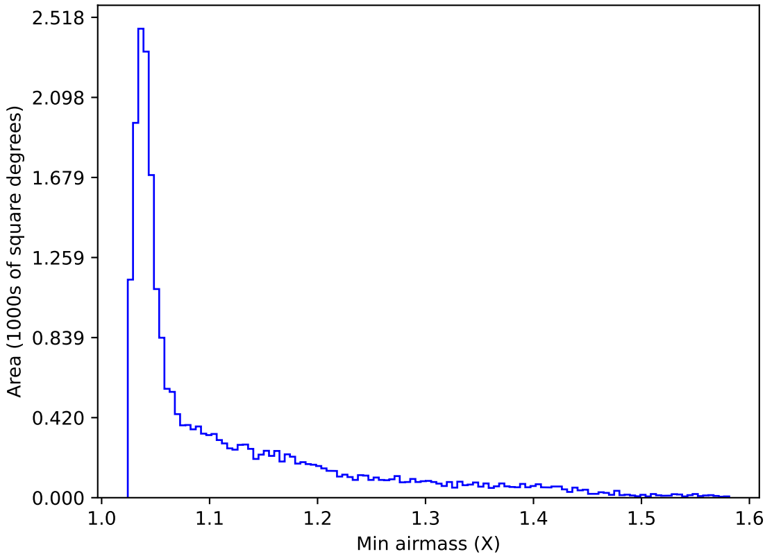
noroll_mjdp120_v3.4_10yrs All sky u band: Min airmass
