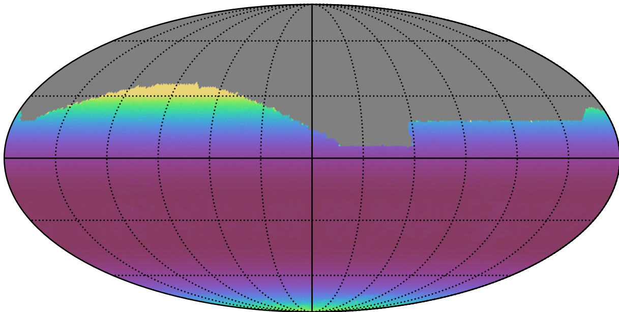
noroll_mjdp120_v3.4_10yrs All sky r band: Min airmass
