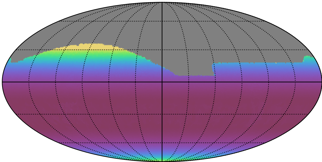
noroll_mjdp120_v3.4_10yrs All sky i band: Min airmass
