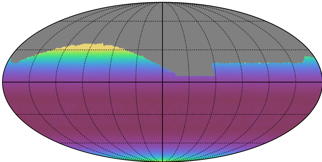
noroll_mjdp120_v3.4_10yrs All sky g band: Min airmass
