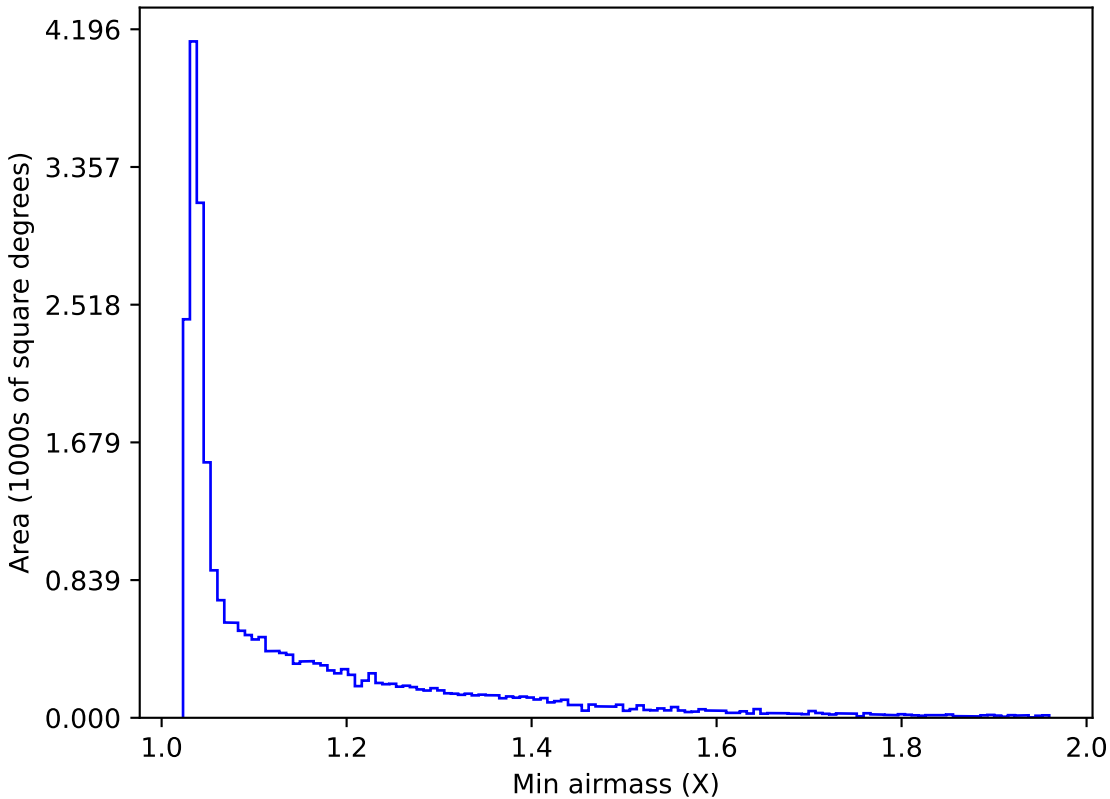
noroll_mjdp120_v3.4_10yrs All sky g band: Min airmass
