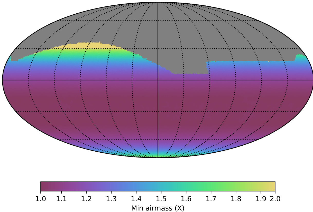
noroll_mjdp120_v3.4_10yrs All sky all bands: Min airmass
