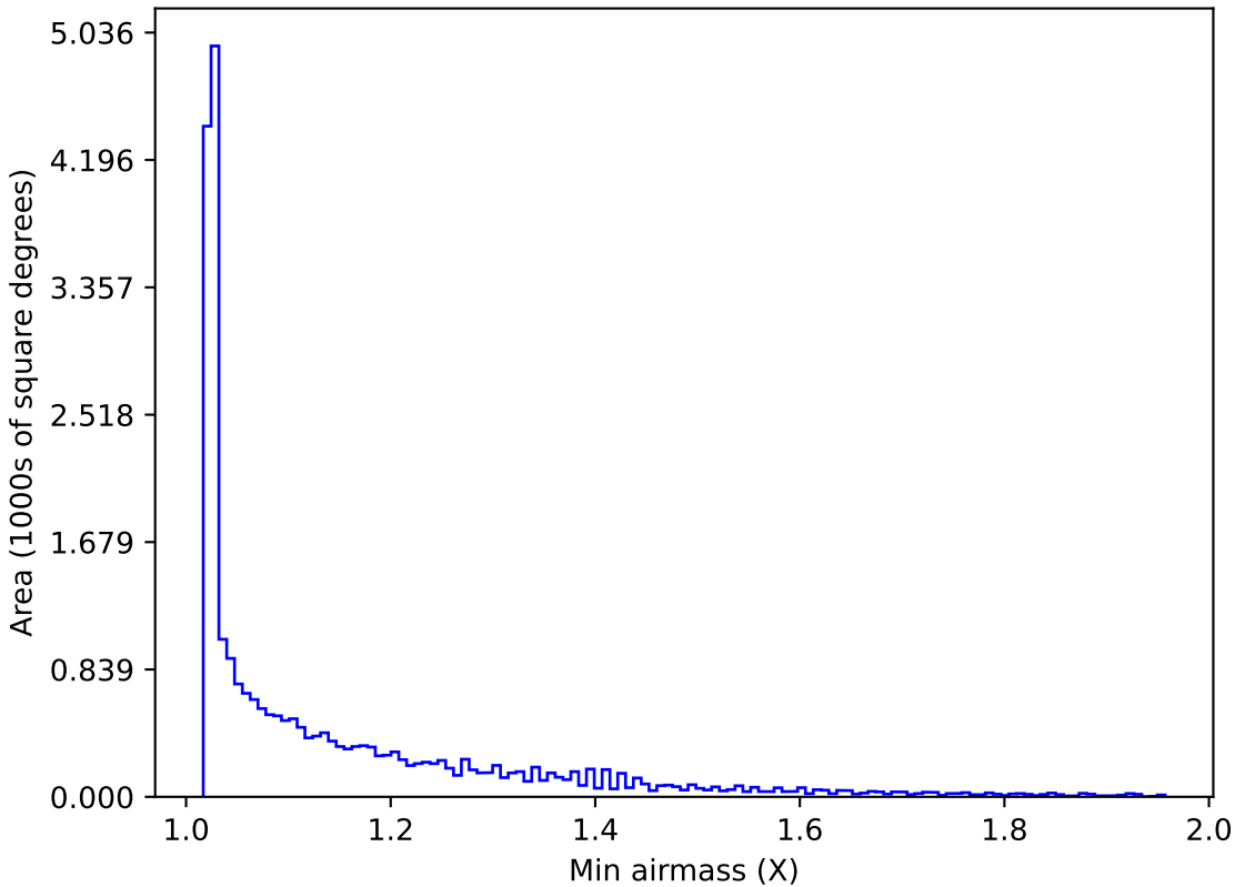
noroll_mjdp120_v3.4_10yrs All sky all bands: Min airmass
