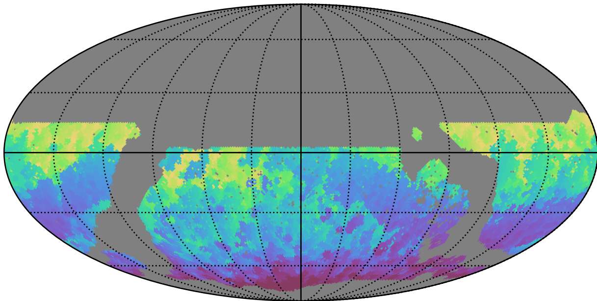
noroll_mjdp120_v3.4_10yrs WFD z band: Min HA
