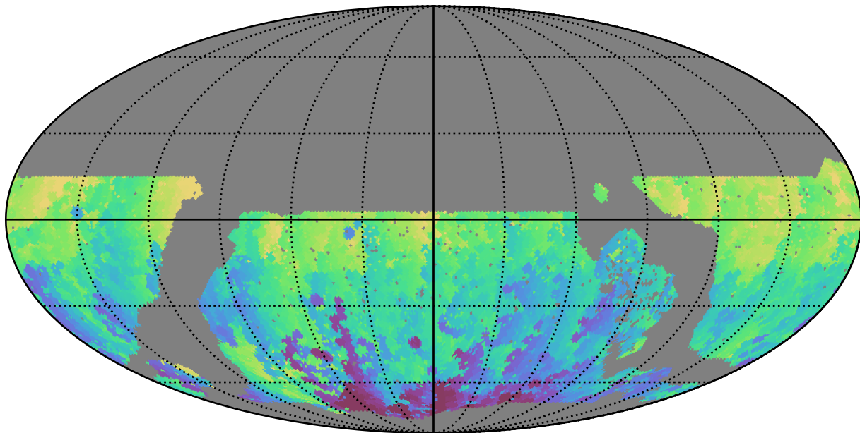
noroll_mjdp120_v3.4_10yrs WFD u band: Min HA
