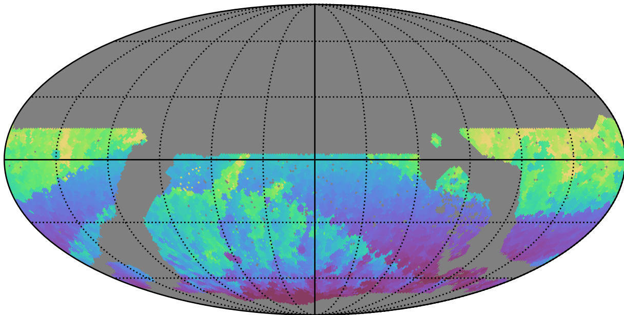
noroll_mjdp120_v3.4_10yrs WFD r band: Min HA
