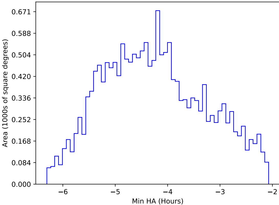
noroll_mjdp120_v3.4_10yrs WFD r band: Min HA
