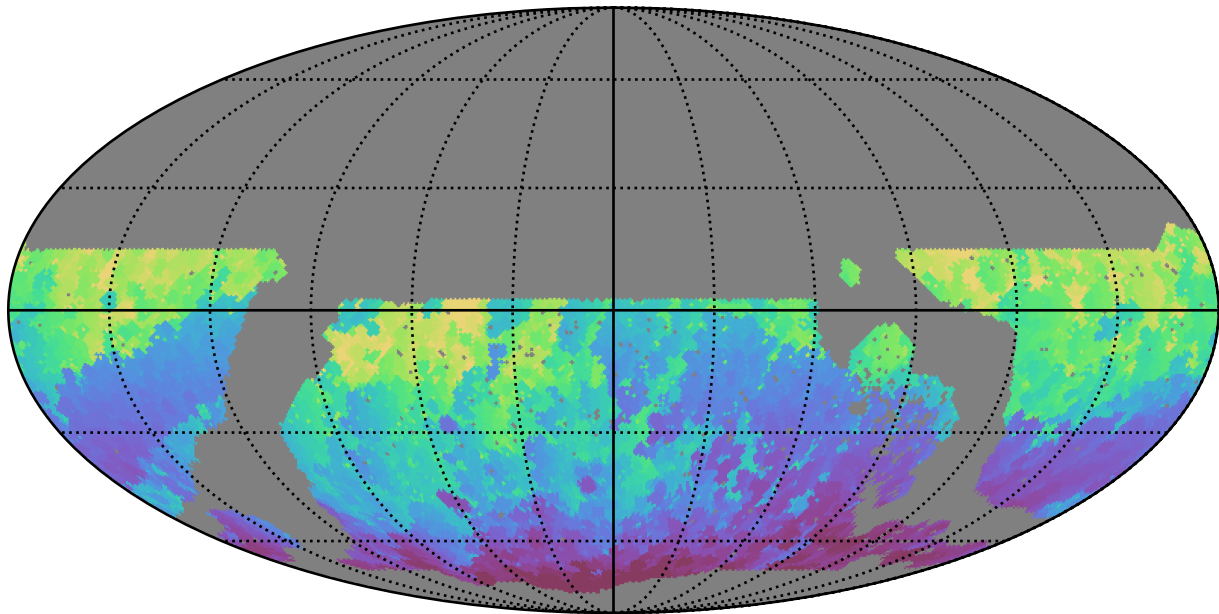
noroll_mjdp120_v3.4_10yrs WFD i band: Min HA
