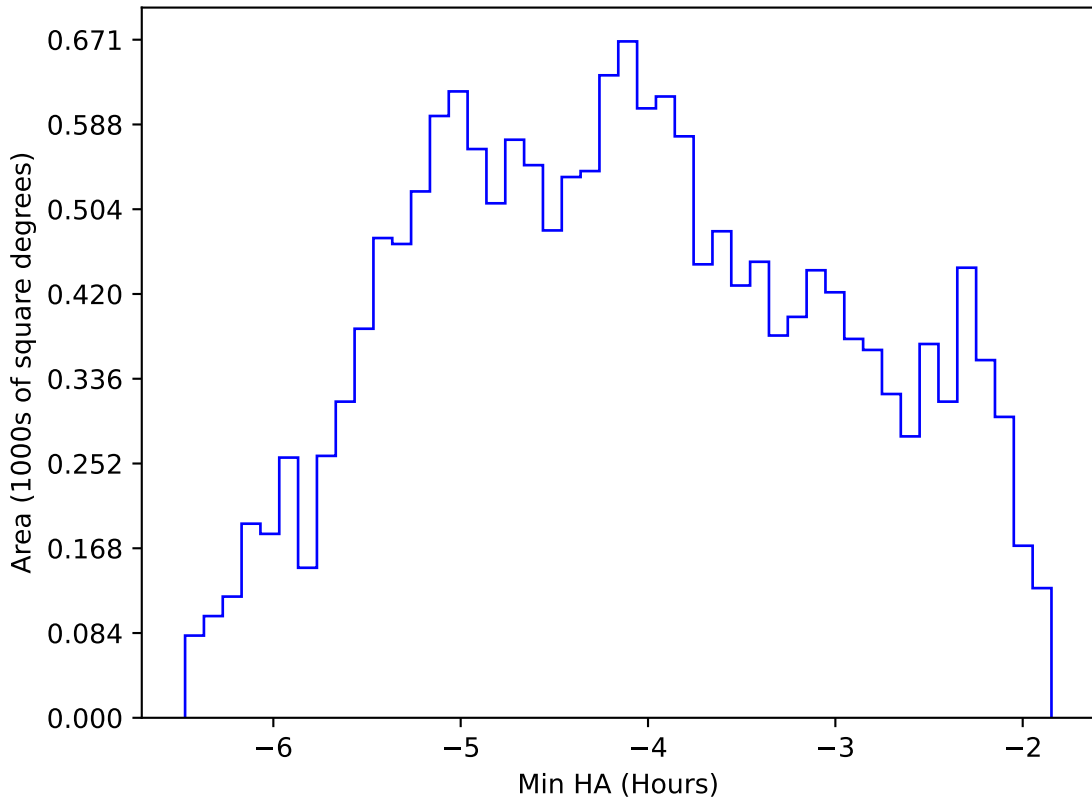
noroll_mjdp120_v3.4_10yrs WFD i band: Min HA
