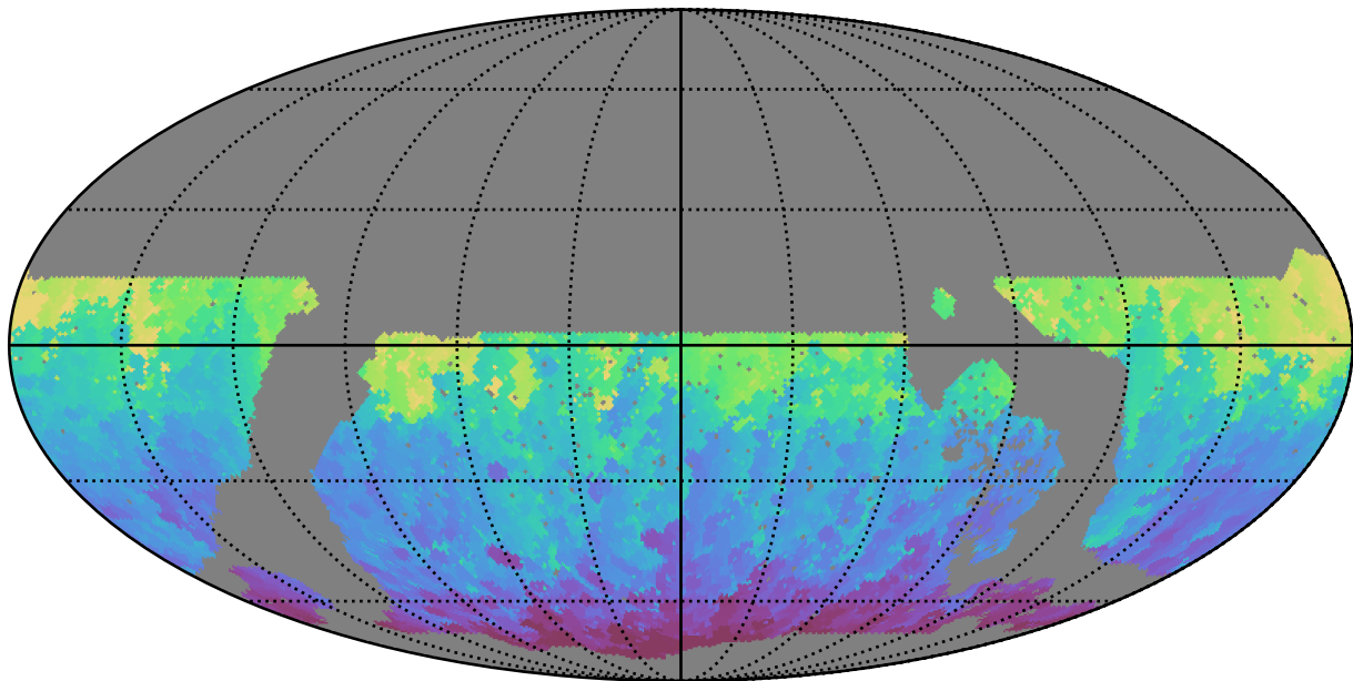
noroll_mjdp120_v3.4_10yrs WFD g band: Min HA
