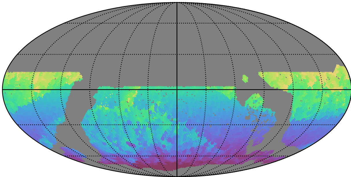
noroll_mjdp120_v3.4_10yrs WFD all bands: Min HA
