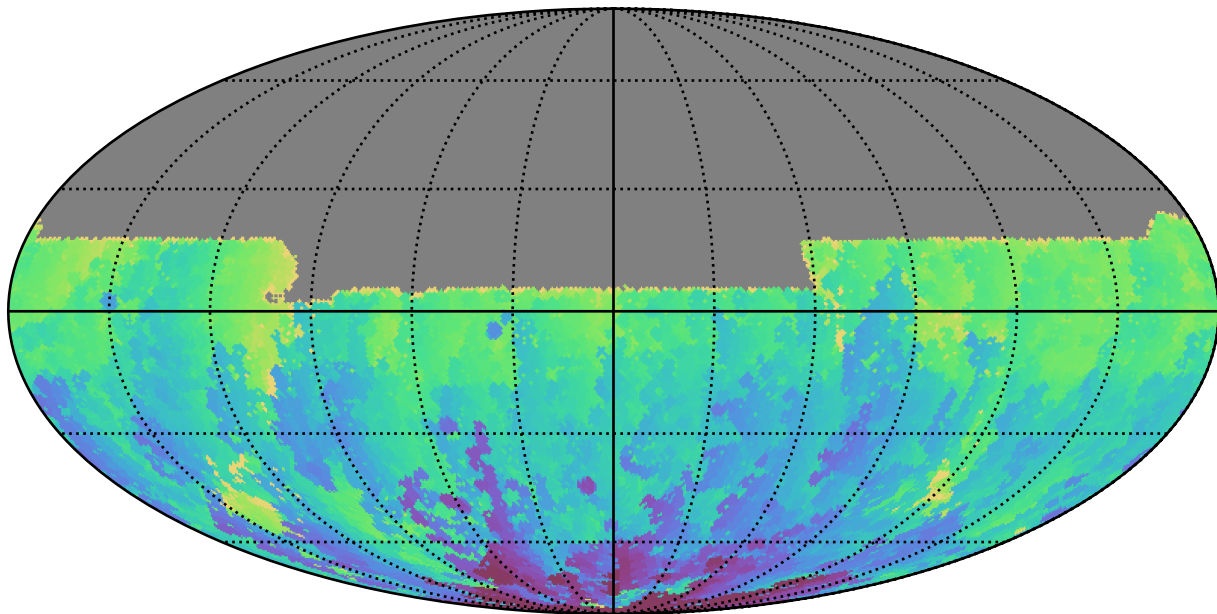
noroll_mjdp120_v3.4_10yrs All sky u band: Min HA
