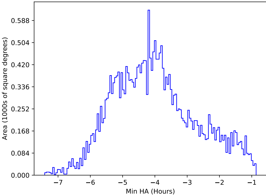
noroll_mjdp120_v3.4_10yrs All sky r band: Min HA
