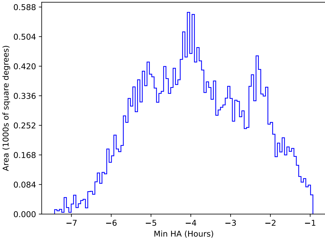
noroll_mjdp120_v3.4_10yrs All sky i band: Min HA
