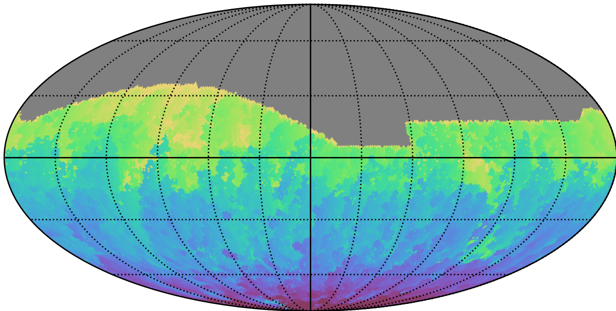
noroll_mjdp120_v3.4_10yrs All sky g band: Min HA
