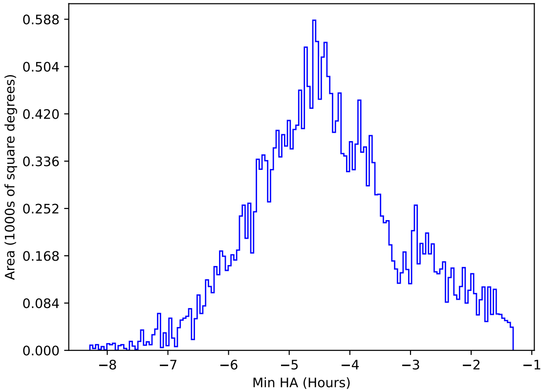
noroll_mjdp120_v3.4_10yrs All sky all bands: Min HA
