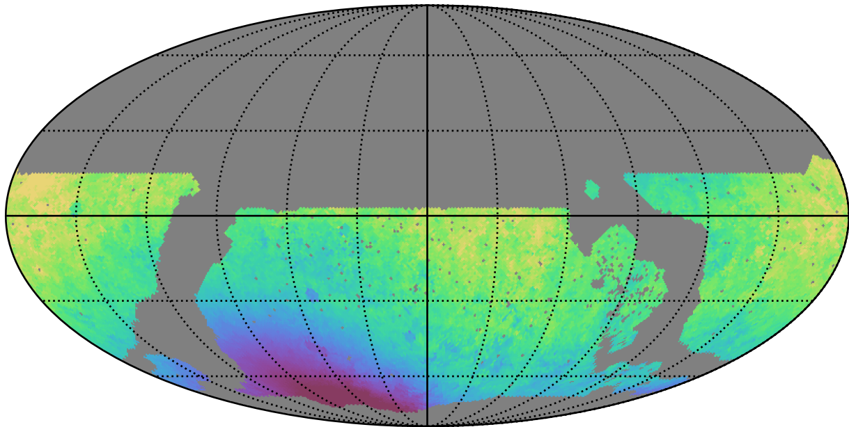
noroll_mjdp120_v3.4_10yrs WFD z band: Median solarElong
