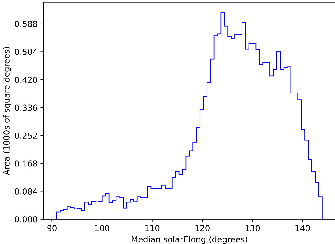
noroll_mjdp120_v3.4_10yrs WFD z band: Median solarElong
