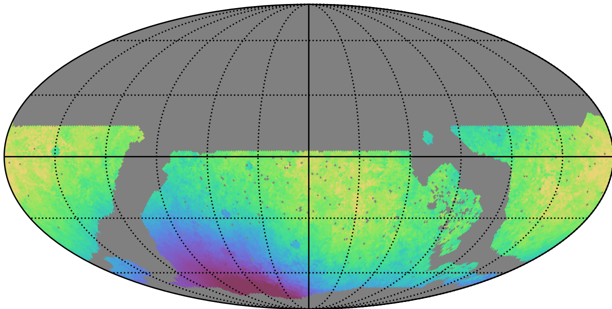
noroll_mjdp120_v3.4_10yrs WFD y band: Median solarElong
