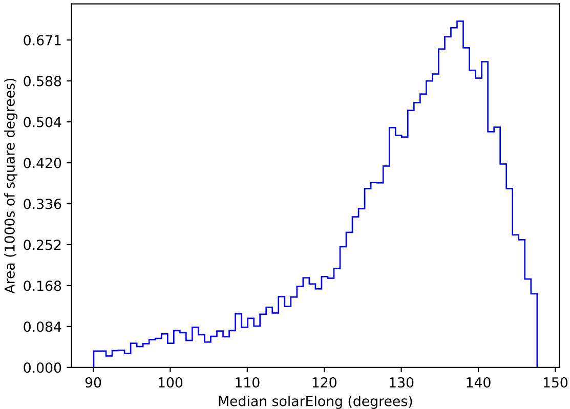
noroll_mjdp120_v3.4_10yrs WFD y band: Median solarElong
