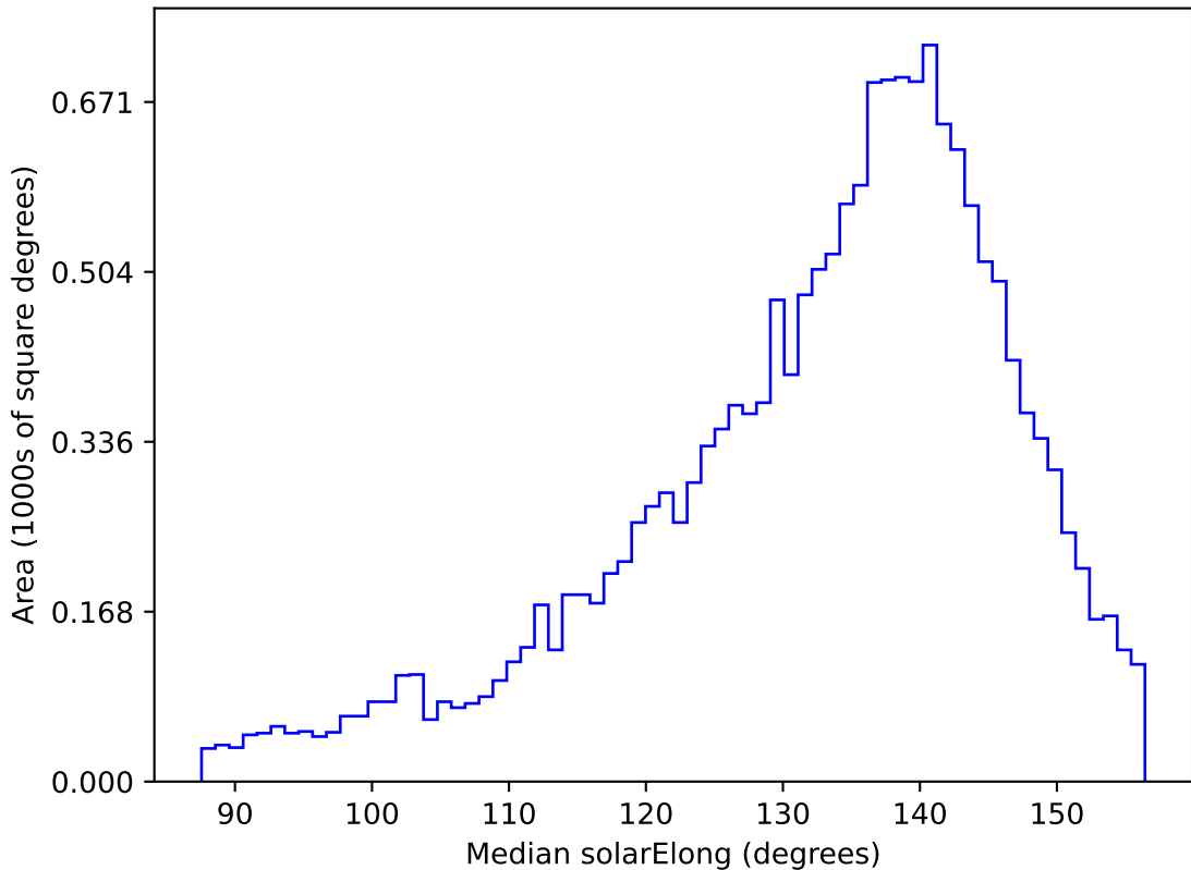
noroll_mjdp120_v3.4_10yrs WFD u band: Median solarElong
