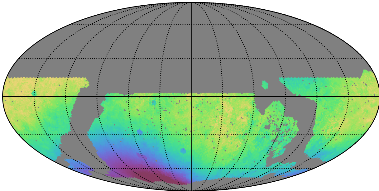
noroll_mjdp120_v3.4_10yrs WFD r band: Median solarElong
