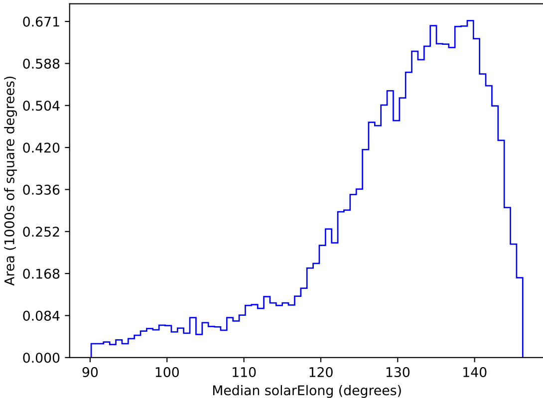
noroll_mjdp120_v3.4_10yrs WFD r band: Median solarElong
