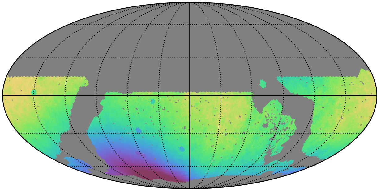
noroll_mjdp120_v3.4_10yrs WFD all bands: Median solarElong
