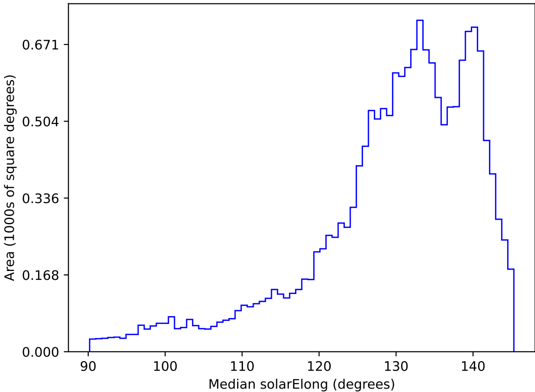
noroll_mjdp120_v3.4_10yrs WFD all bands: Median solarElong
