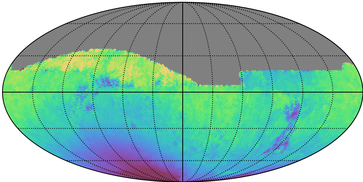
noroll_mjdp120_v3.4_10yrs All sky z band: Median solarElong
