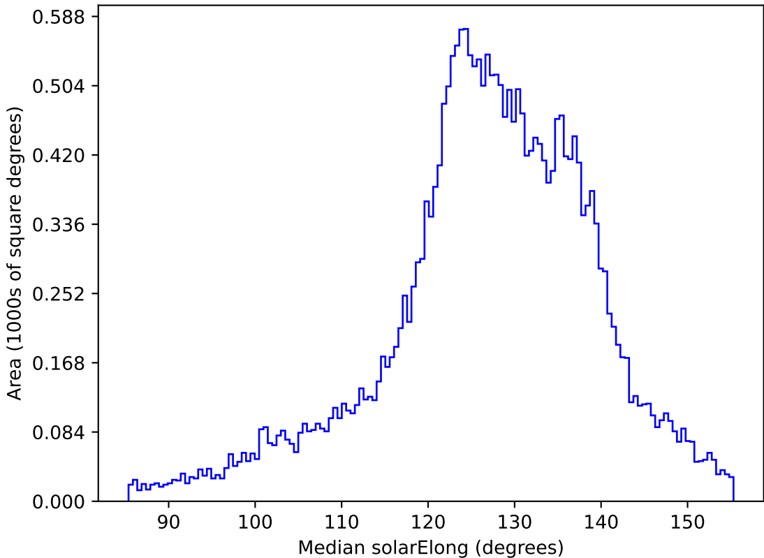
noroll_mjdp120_v3.4_10yrs All sky z band: Median solarElong
