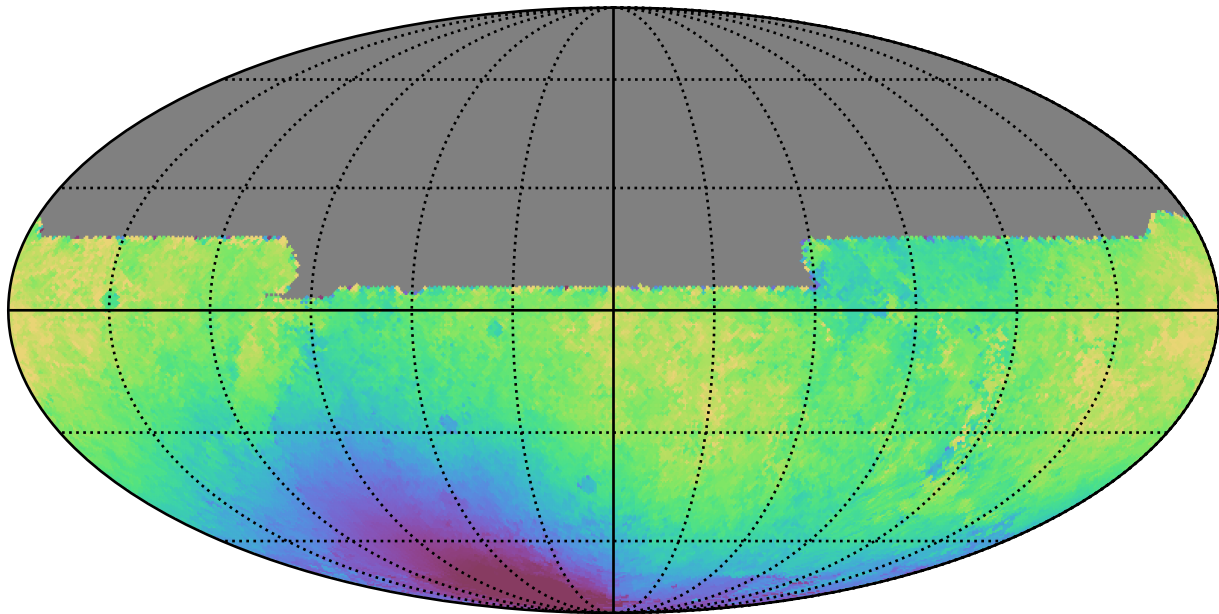
noroll_mjdp120_v3.4_10yrs All sky y band: Median solarElong
