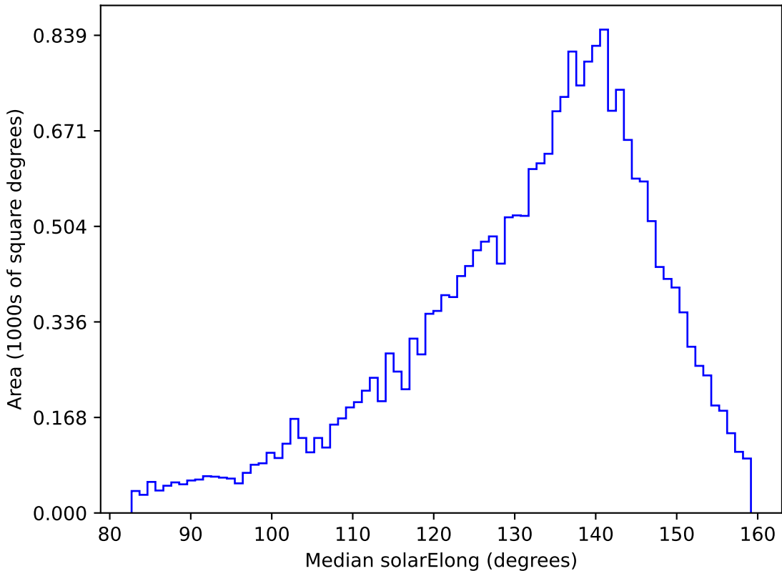
noroll_mjdp120_v3.4_10yrs All sky u band: Median solarElong
