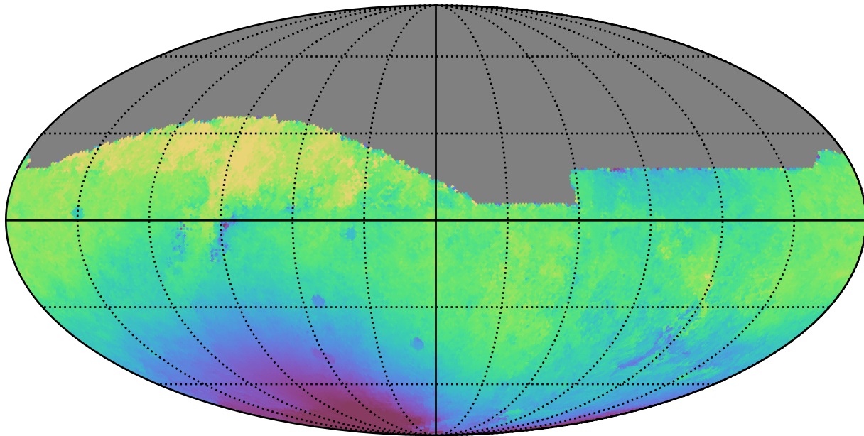
noroll_mjdp120_v3.4_10yrs All sky r band: Median solarElong
