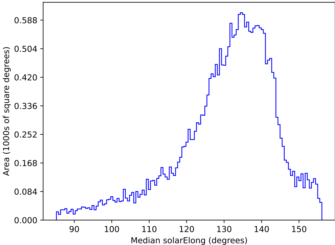
noroll_mjdp120_v3.4_10yrs All sky r band: Median solarElong
