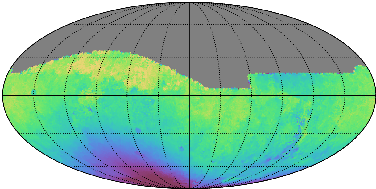
noroll_mjdp120_v3.4_10yrs All sky i band: Median solarElong
