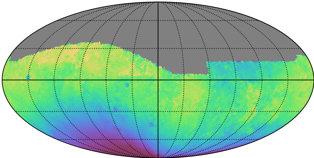
noroll_mjdp120_v3.4_10yrs All sky g band: Median solarElong
