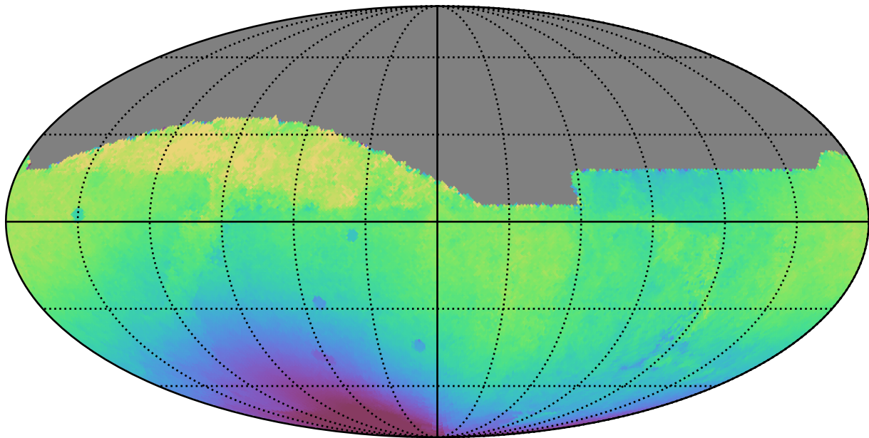
noroll_mjdp120_v3.4_10yrs All sky all bands: Median solarElong
