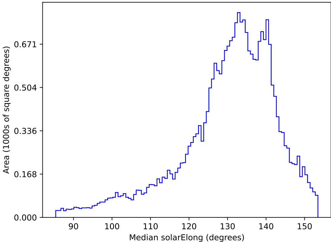
noroll_mjdp120_v3.4_10yrs All sky all bands: Median solarElong
