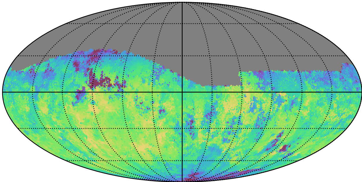
noroll_mjdp120_v3.4_10yrs Yr 1 z band: Median skyBrightness
