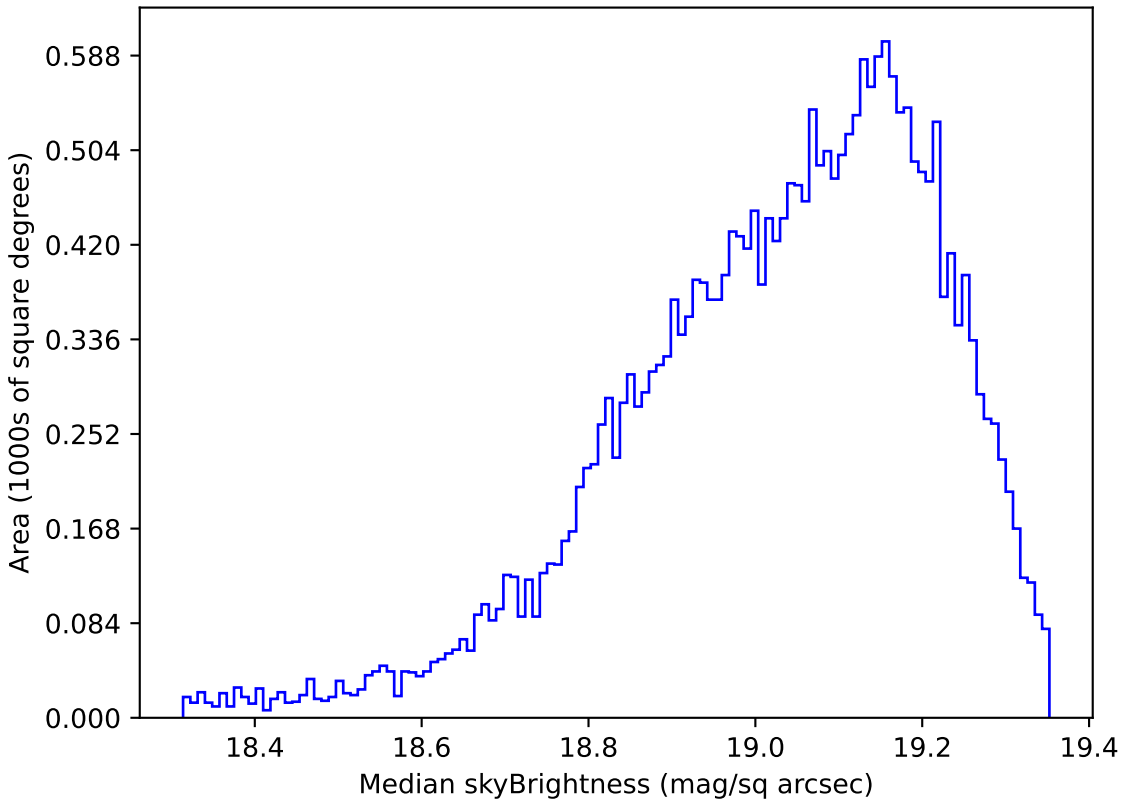
noroll_mjdp120_v3.4_10yrs Yr 1 z band: Median skyBrightness
