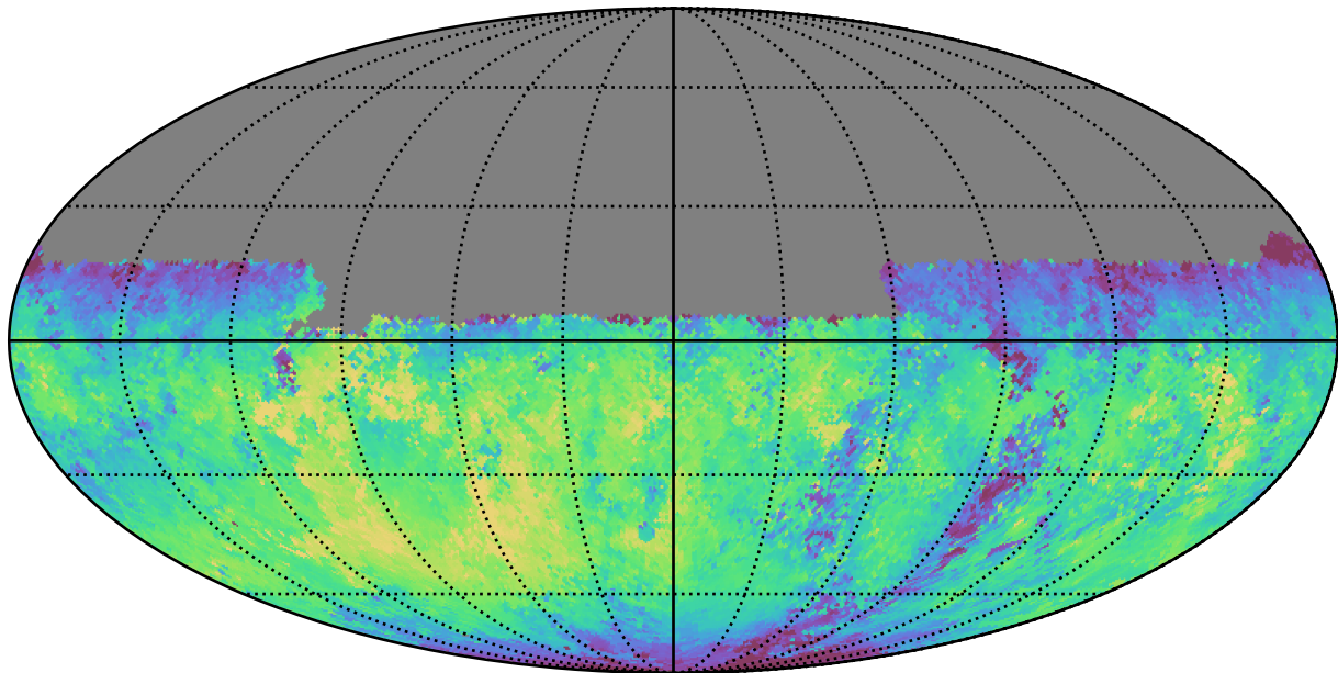
noroll_mjdp120_v3.4_10yrs Yr 1 y band: Median skyBrightness
