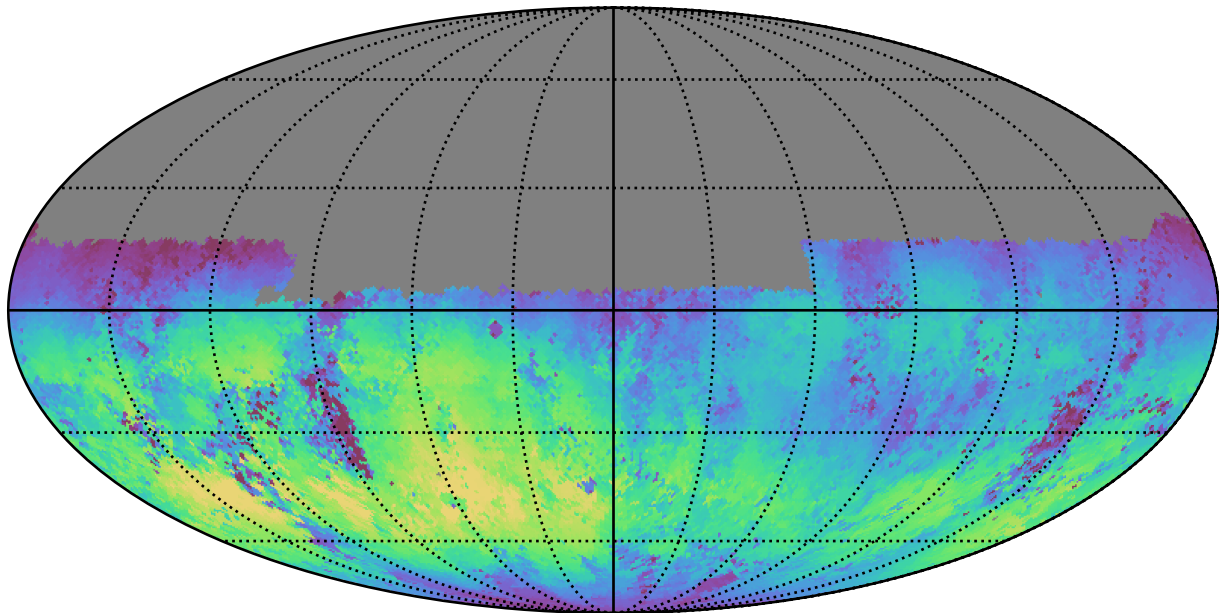
noroll_mjdp120_v3.4_10yrs Yr 1 u band: Median skyBrightness
